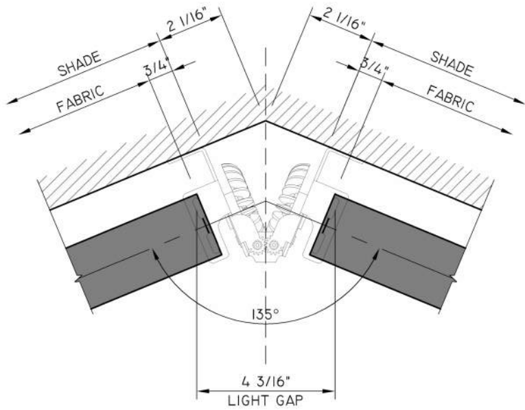
ANGLE COUPLER SHOWING 135° ANGLE
